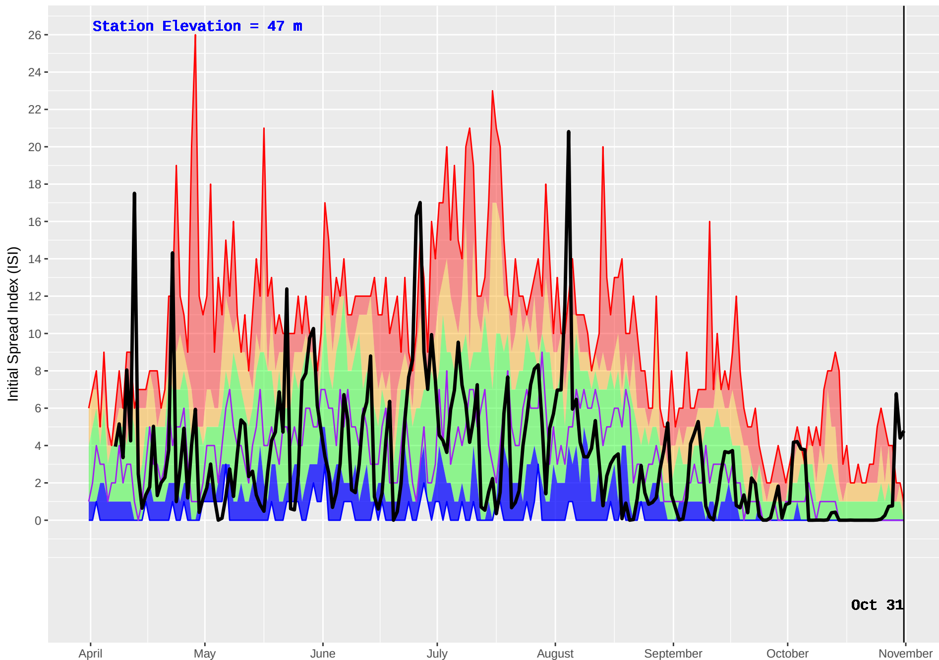
HAGENSBORG 2 (904) : Historical (2005–2016) and Current (2017) Noon Initial Spread Index (ISI)
