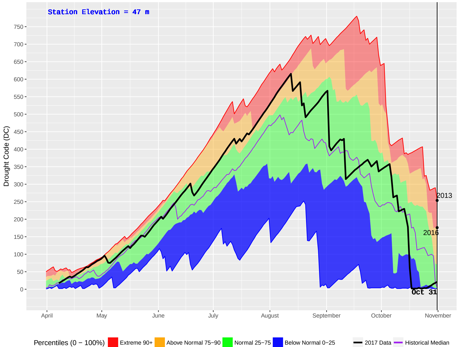
HAGENSBORG 2 (904) : Historical (2005–2016) and Current (2017) Noon Drought Code (DC)
