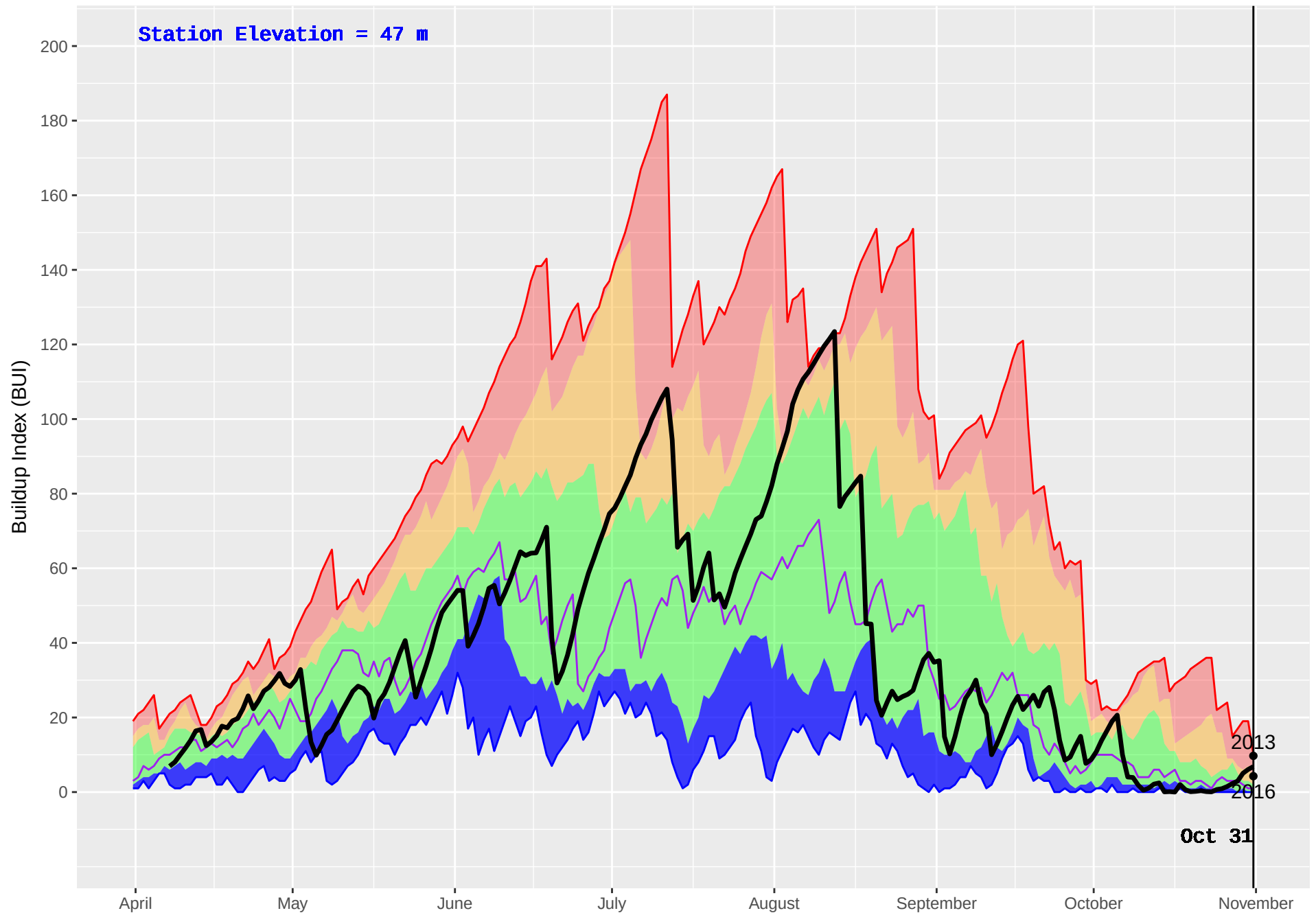
HAGENSBORG 2 (904) : Historical (2005–2016) and Current (2017) Noon Buildup Index (BUI)
